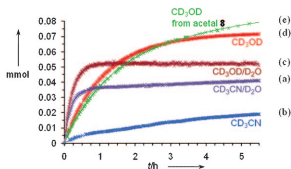
Figure 1. Relative rates of iminium ion formation: a) Cinnamaldehyde ( 7 ) in CD 3 CN/D 2 O (19:1) 1 M, 25 °C, 20 mol% 1 ·HCl (purple trace); b) cinnamaldehyde ( 7 ) in CD 3 CN 1 M, 25 °C, 20 mol% 1 ·HCl (blue trace); c) cinnamaldehyde ( 7 ) in CD 3 OD/D 2 O (19:1) 1 M, 25 °C, 20 mol% 1 ·HCl (dark red trace); d) cinnamaldehyde ( 7 ) in CD 3 OD 1 M, 25 °C, 20 mol% 1 ·HCl (red trace); e) cinnamaldehyde dimethyl acetal ( 8 ) in CD 3 OD 1 M, 25 °C, 20 mol% 1 ·HCl (green trace).
